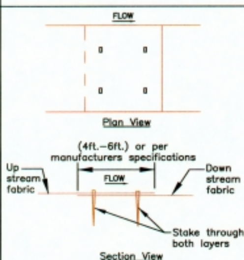
SECTION B - B': FABRIC END JOINT DETAILS
