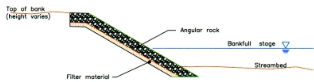
TYPICAL RIPRAP WITH EXCAVATED TOE
