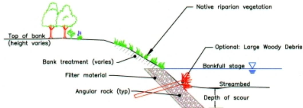
EXCAVATED TOE
