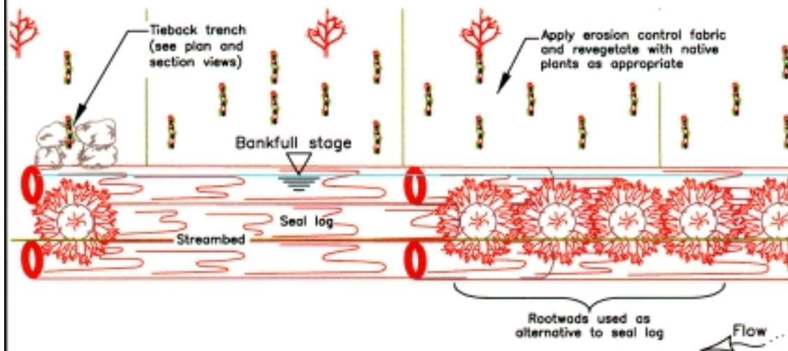
ELEVATION VIEW FROM RIVER
