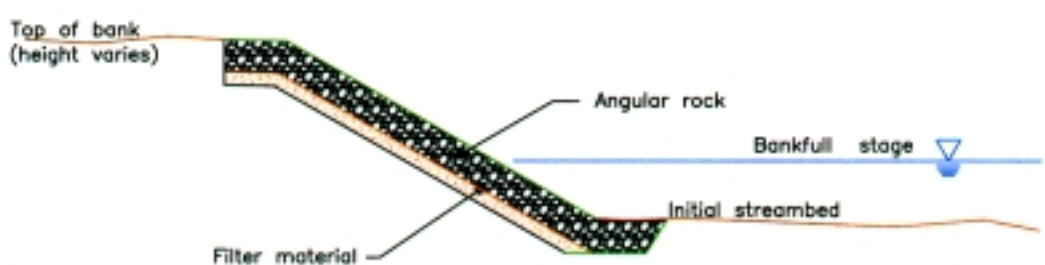
LAUNCHABLE TOE (Before toe is launched into scour hole)
