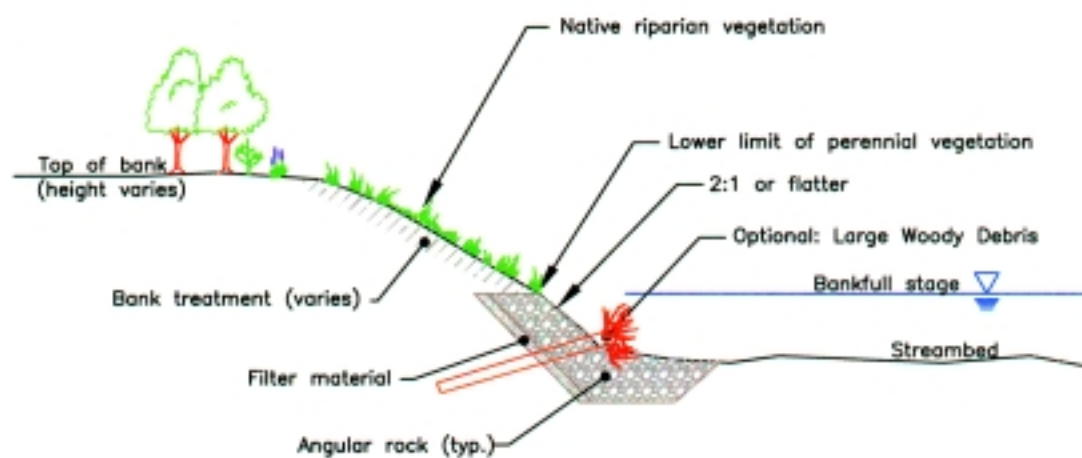
LAUNCHABLE TOE
